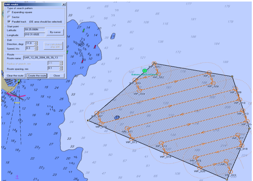
Example of a Parallel Line Search Pattern
