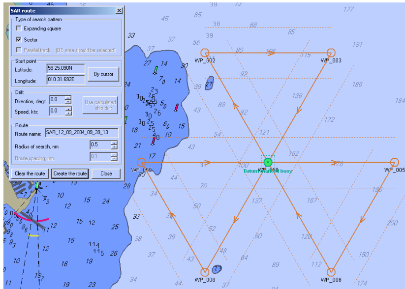
Example of a Sector Search Pattern
