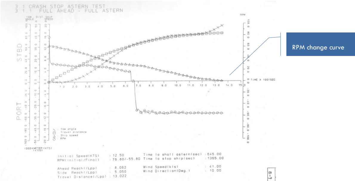
Crash Stop data (from Sea Trials)
